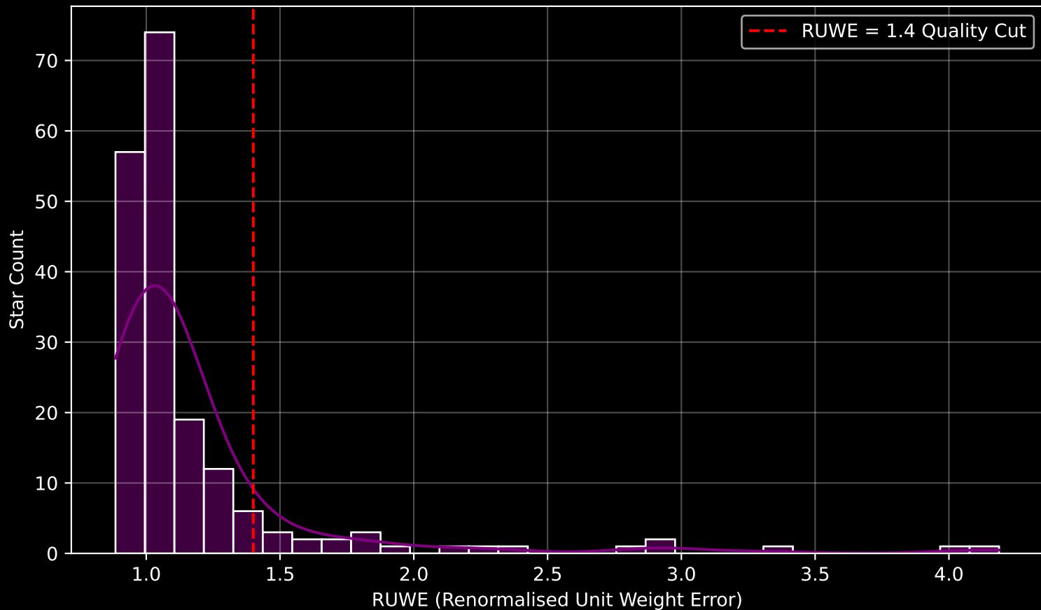
GAPOGEE DR17 Field [325+76] RUWE Distribution (n= 188)
