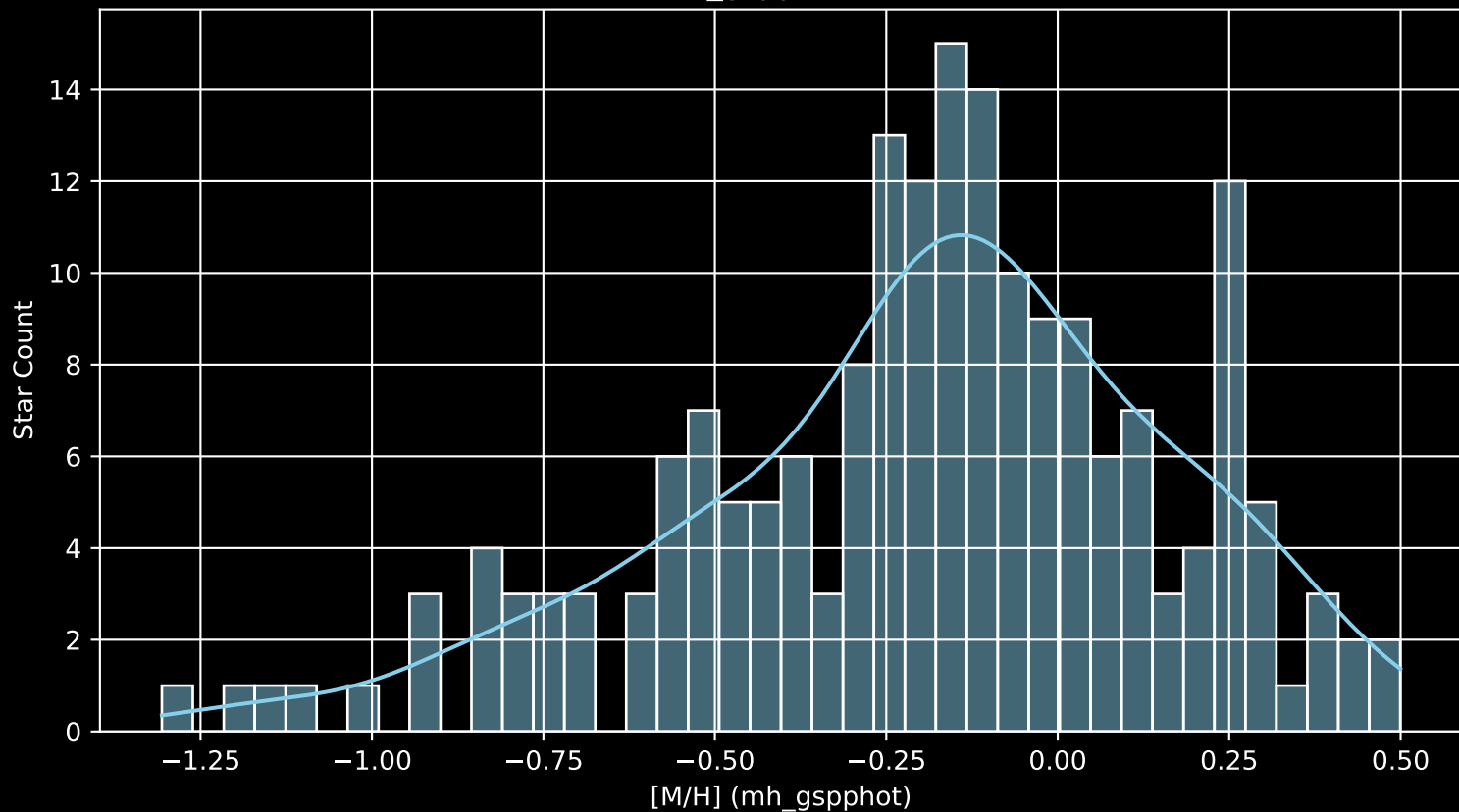
APOGEE DR17 Field: [325+76 [M/H] (mh_gspphot) (n= 191)
