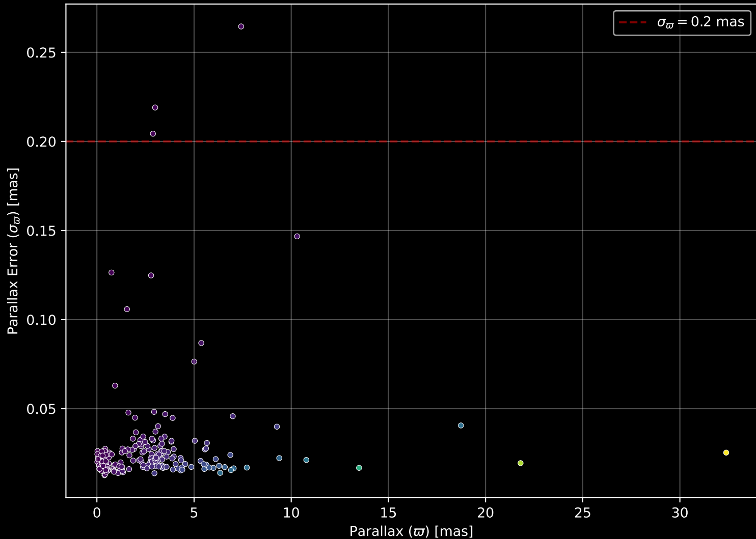
APOGEE DR17 Field: [325+76] Parallax Quality (n= 194)
