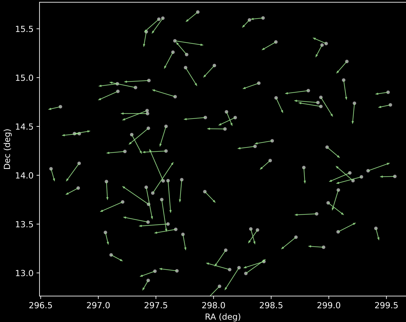
APOGEE DR17 Cluster 5 Proper Motion Vectors (n=91)
