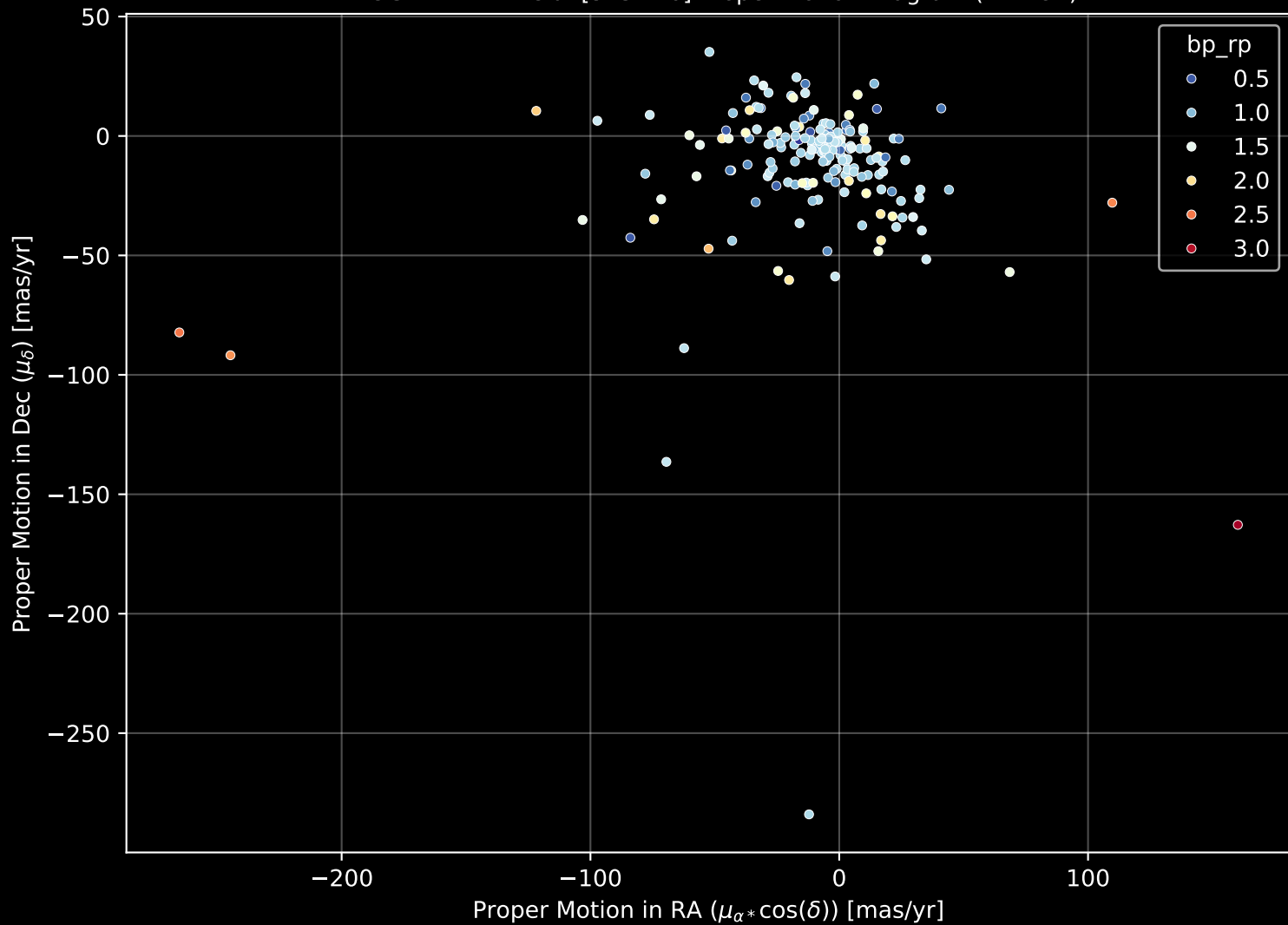
APOGEE DR17 Field: [325+76] Proper Motion Diagram (n= 194)
