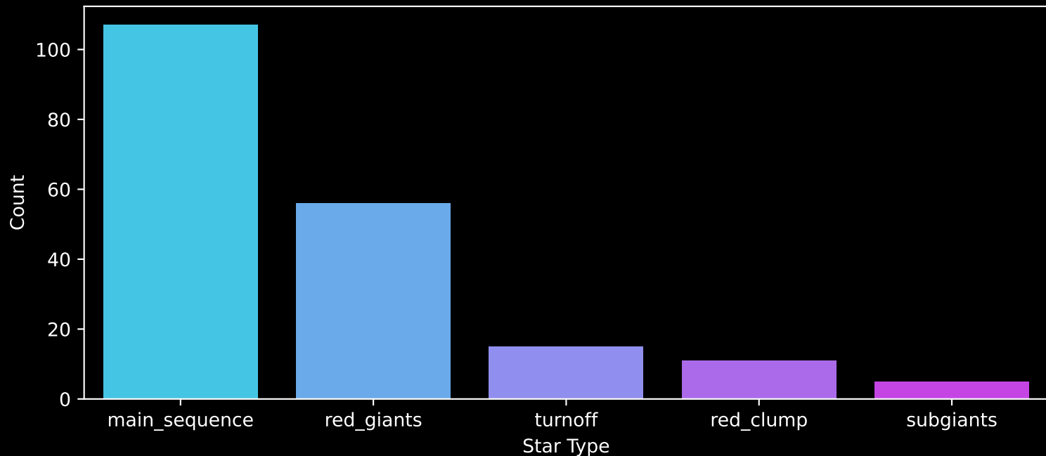
APOGEE DR17 Field: [325+76] Count plot of Star Type
